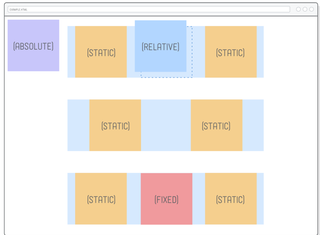
FIXED POSITIONING
