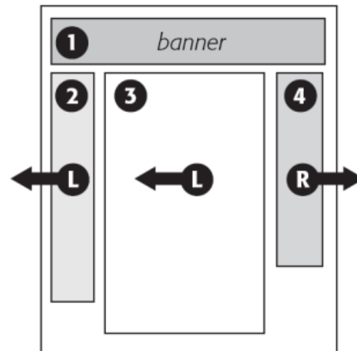
CSS Layout
